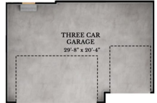
OPTIONAL THREE CAR GARAGE
